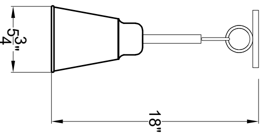
SCH-DSC-LS-18 SMALL LENGTH
