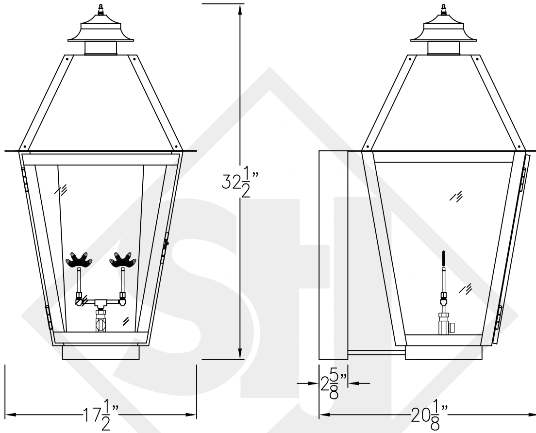
Front View
