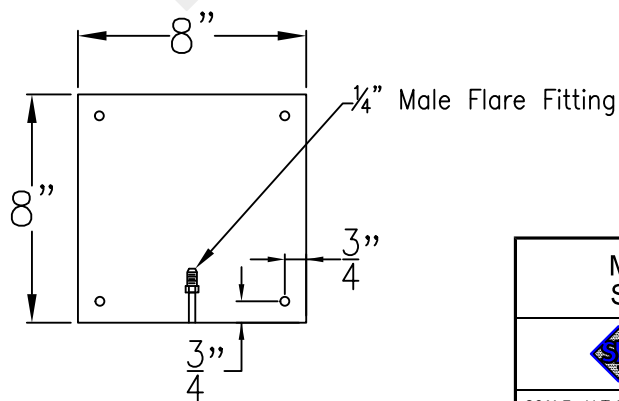
Backplate
