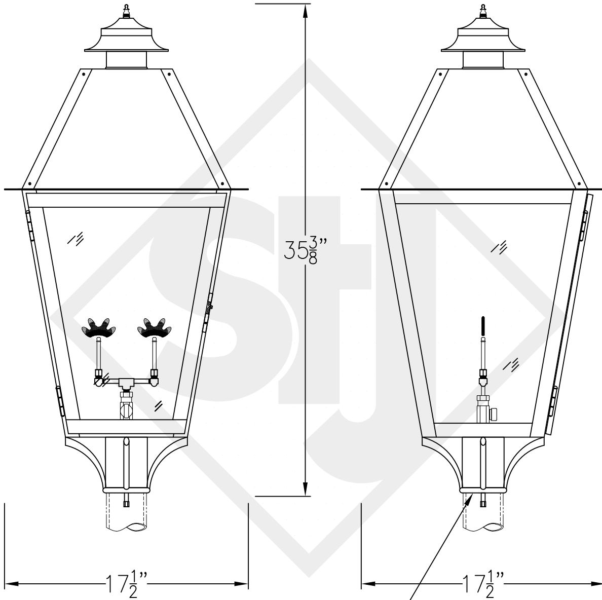
Front View
