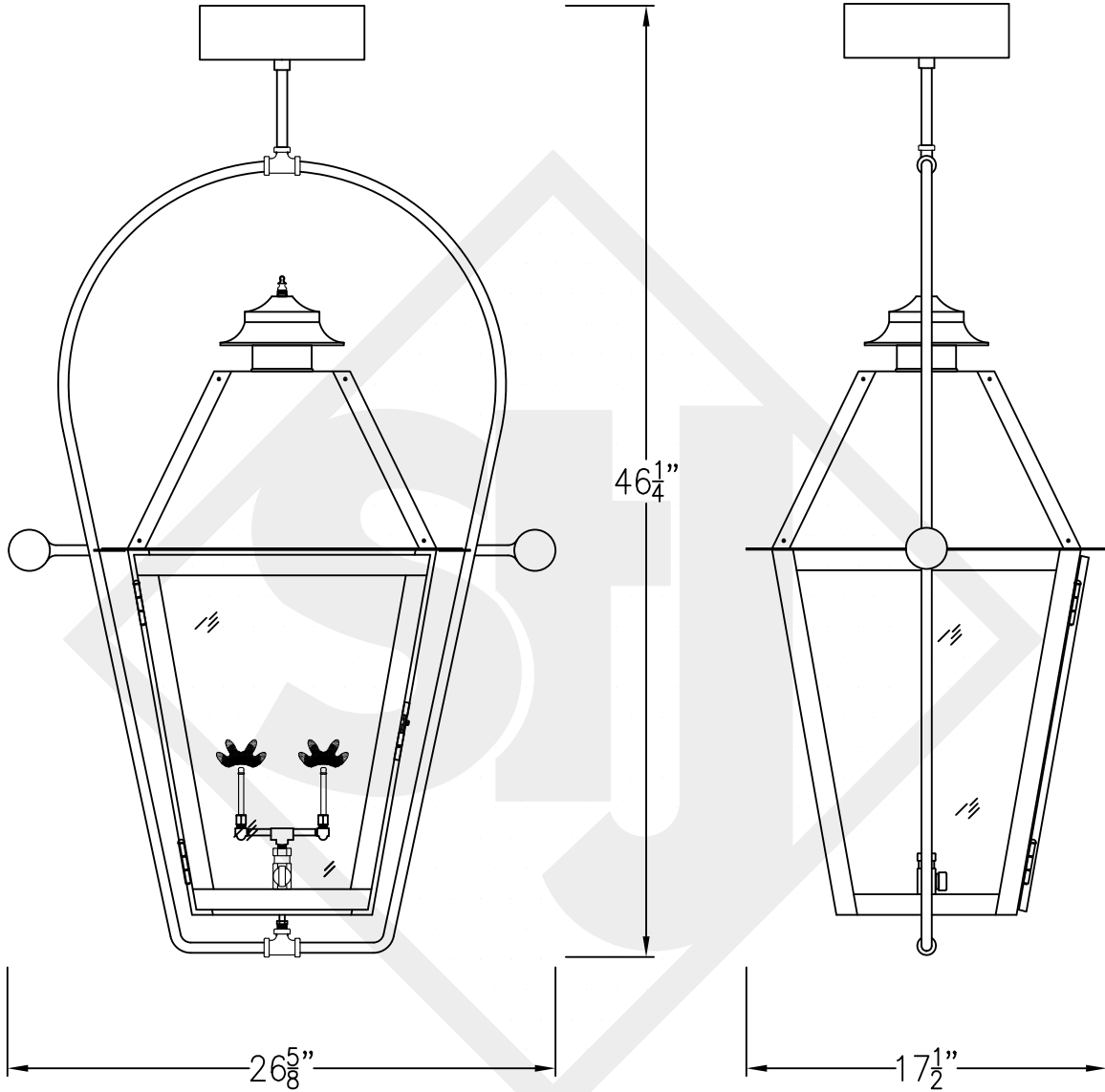
Front View
