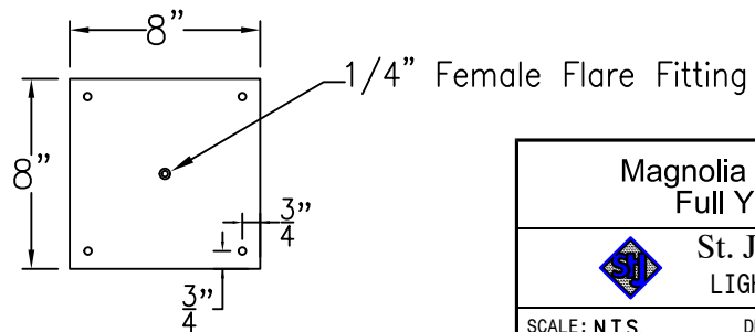
Ceiling Mount
